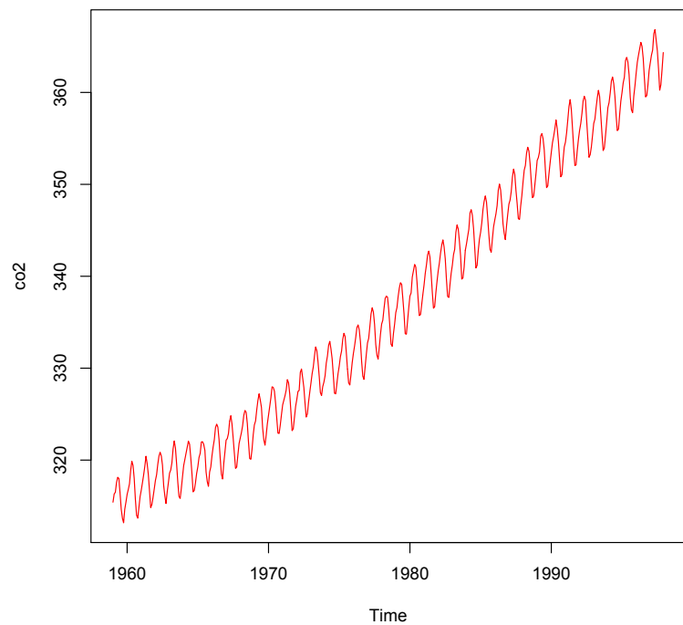
atmospheric [co2] over time
