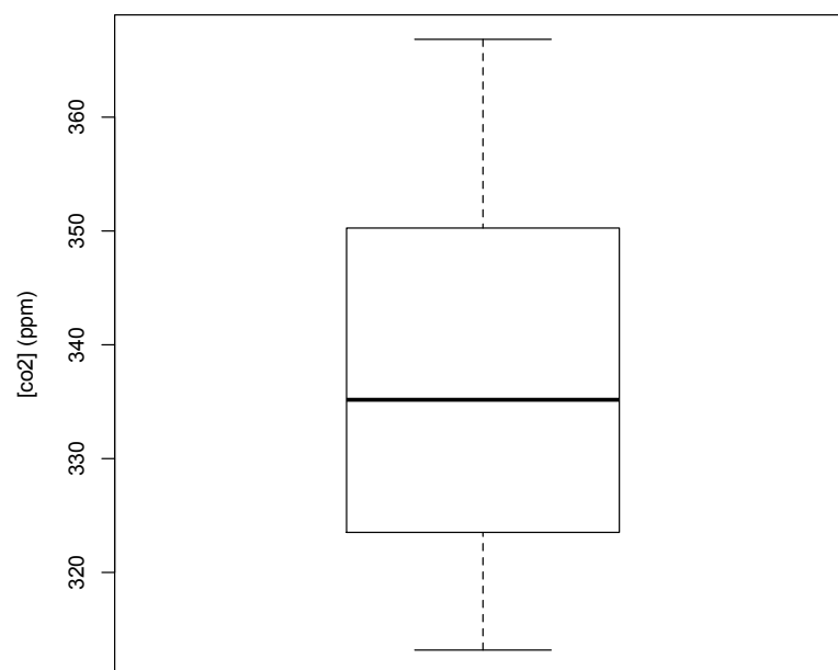
degree of dispersion of [co2]
