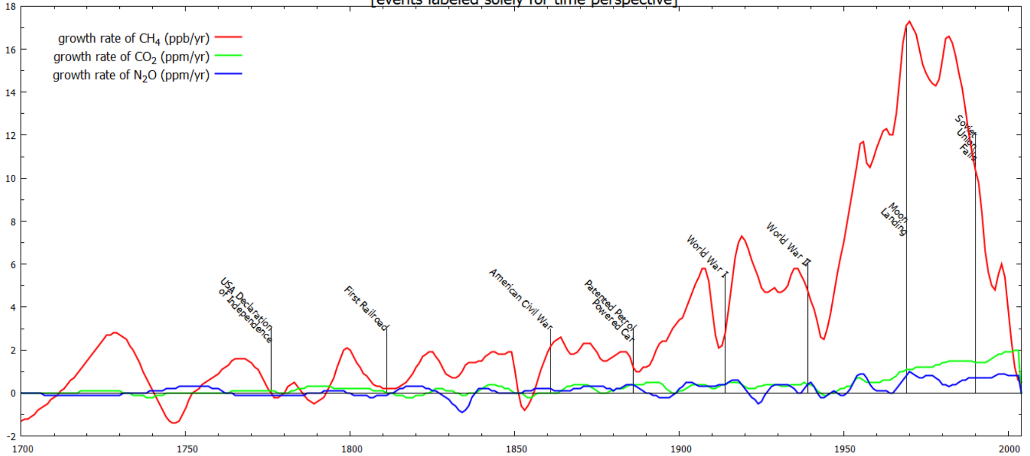
Law Dome Ice Core Data: Growth Rates of CO 2 , CH 4 , and N 2 O [events labeled solely for time perspective]
