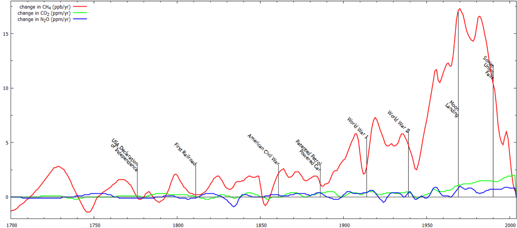
Law Dome Ice Core CO 2 , CH 4 , and N 2 O Data events labeled solely for time perspective
