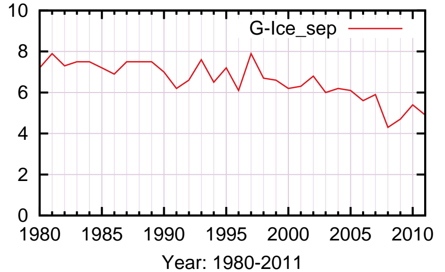
Arctic Sea Ice trend
