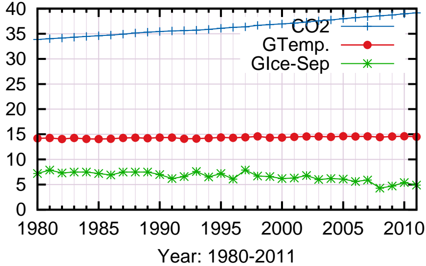
Global Temperature, Sea Ice, CO2 Trend
