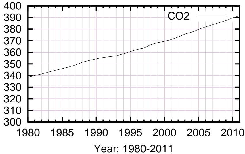
Global CO2 Consumption
