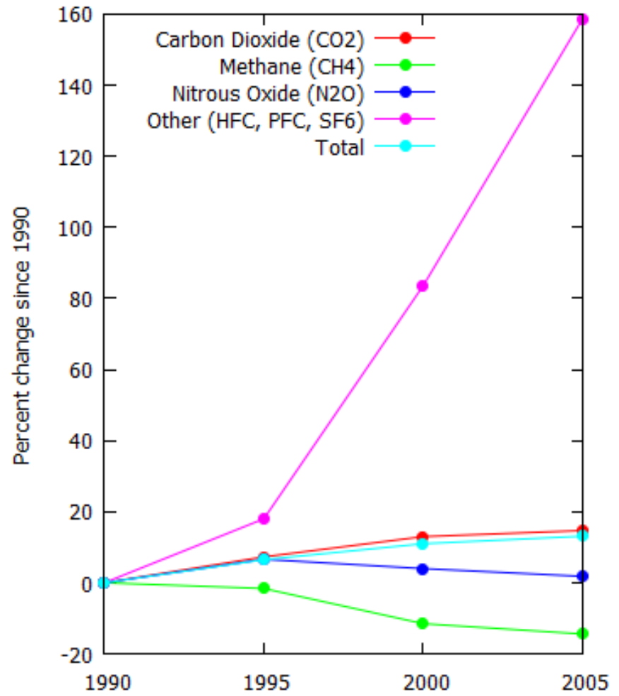
Greenhouse Gas Emissions of United States (1990-2005) Data courtesy of The World Bank
