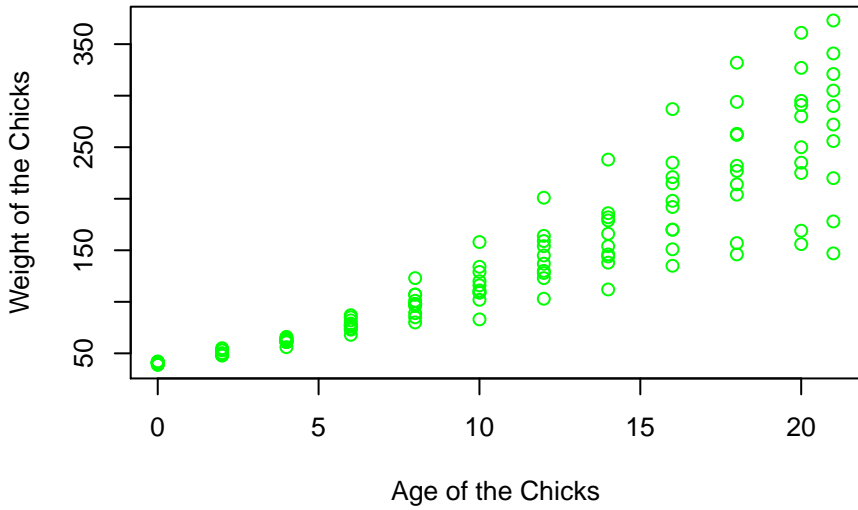
Weight Vs. Age of Chicks on 3 Diets
