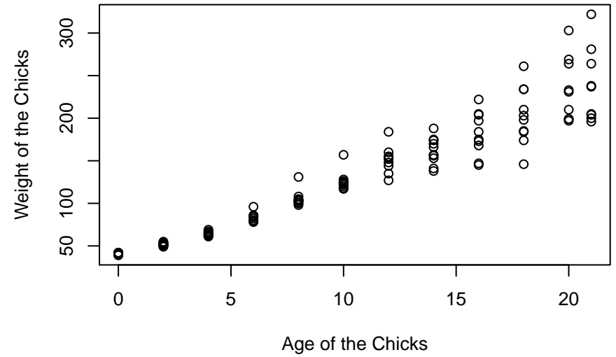
Weight Vs. Age of Chicks on 4 Diets
