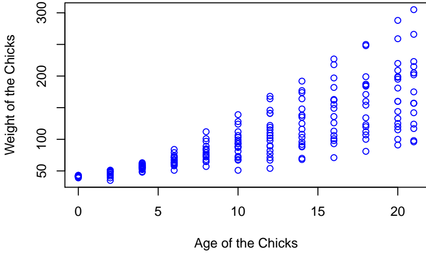
Weight Vs. Age of Chicks on 1 Diets
