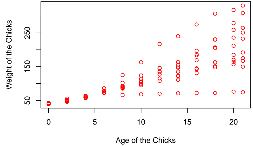
Weight Vs. Age of Chicks on 2 Diets
