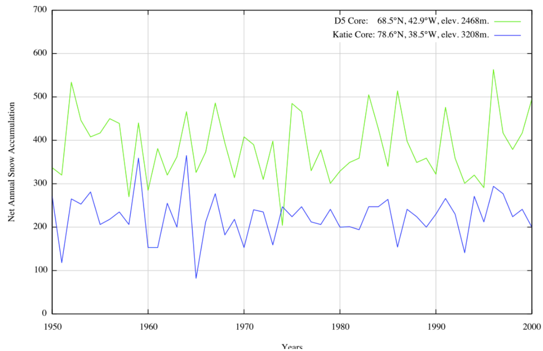
Net Annual Snow Accumulation in Kg - Greenland
