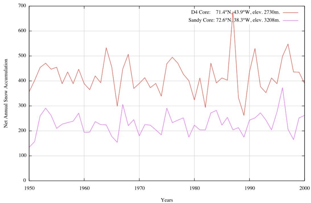
Net Annual Snow Accumulation in Kg - Greenland
